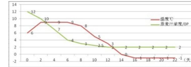
低温发酵工艺曲线 (示例) Graph of Low Temperature Fermentation Process (Demonstration)
